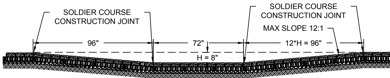
A ADA PARALLEL RAMP PLAN NTS
