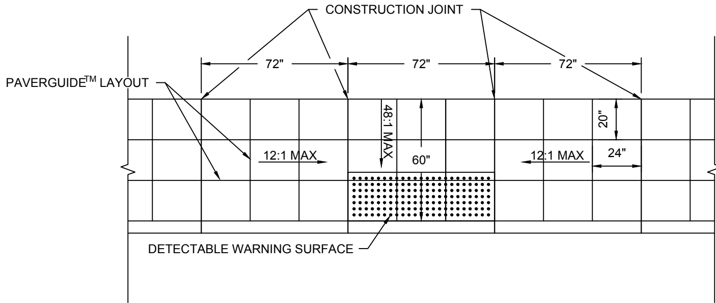
A ADA PARALLEL RAMP PLAN NTS
