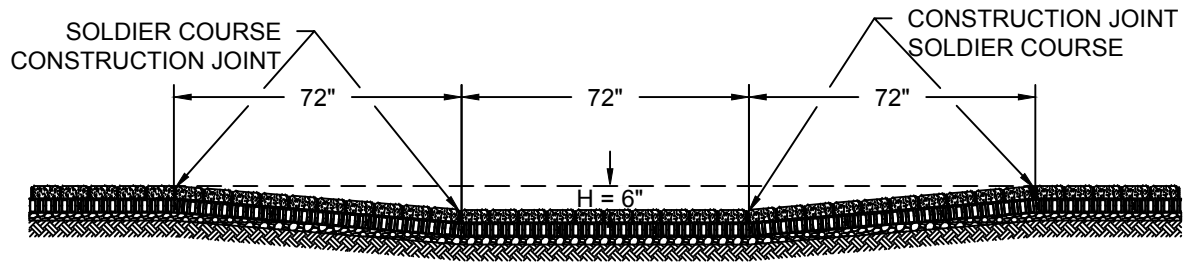
B ADA PARALLEL RAMP ELEVATION NTS
